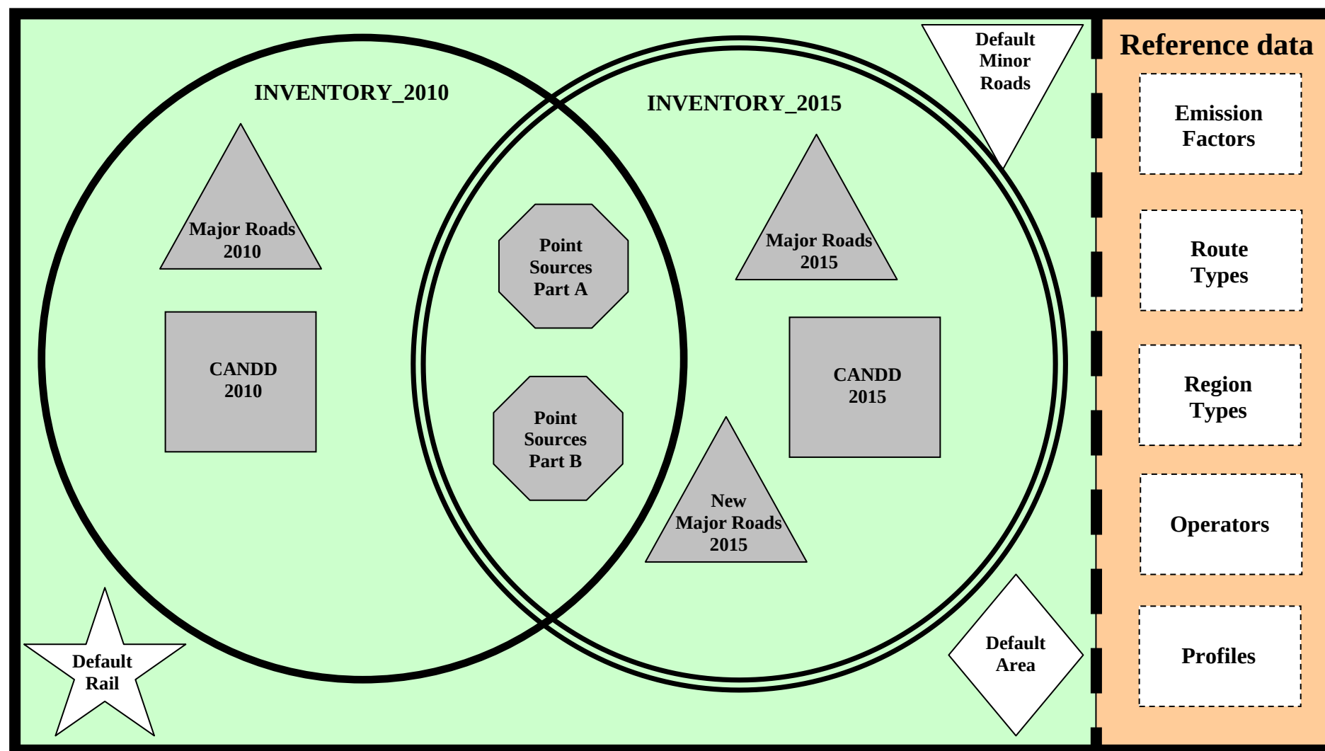
Figure 3.2 – Representation of data hierarchy in EMIT: a database containing inventories which each contain several groups. Each shape represents a different source type. Also in the database are the various 'reference' data, i.e. emission factors, etc
