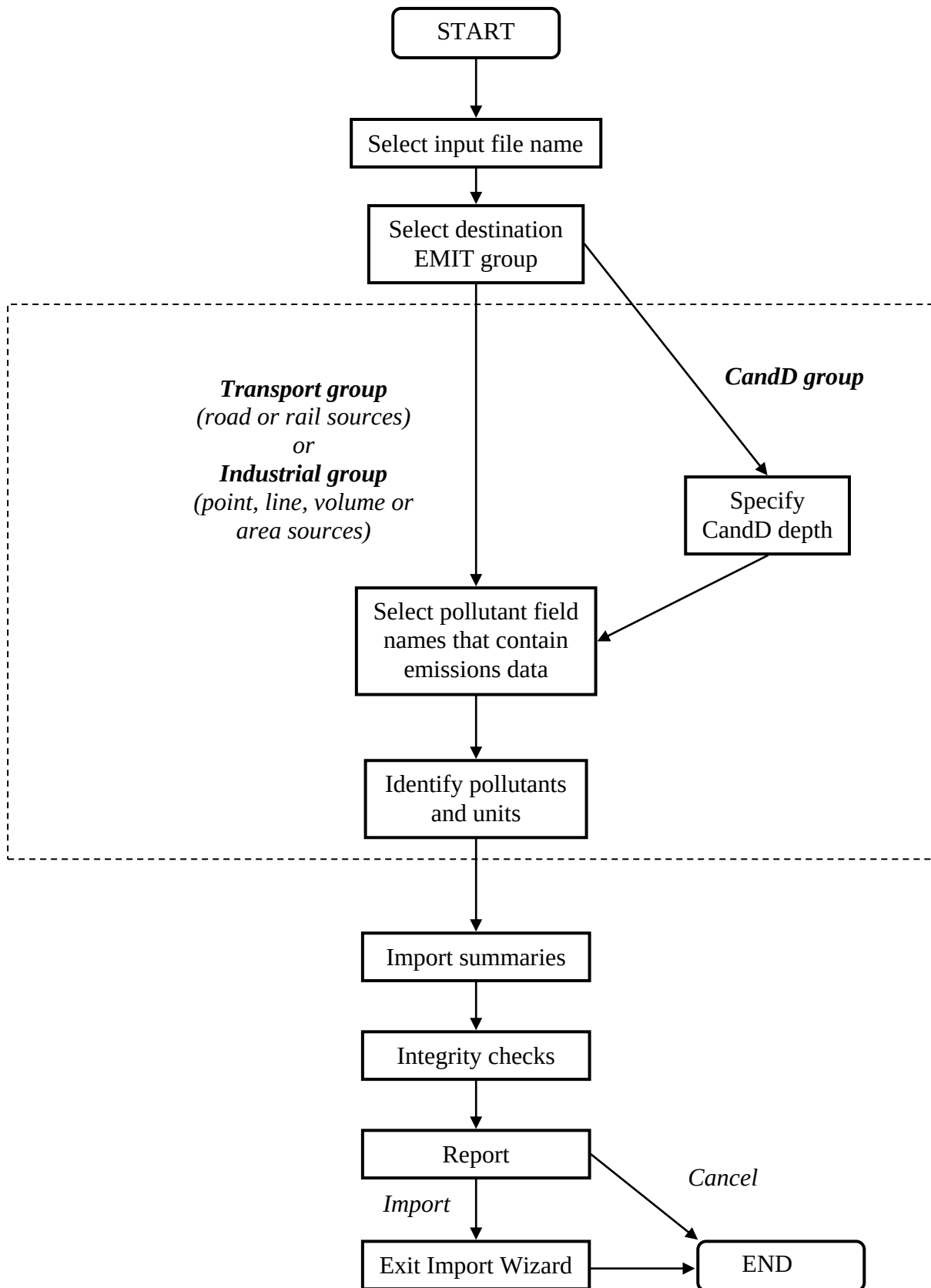
Figure 6.2 – Flow chart showing how to import manually defined emissions data into EMIT using the Import Wizard. Instructions outside the dashed box are in common with Figures 6.3 to 6.5 .
