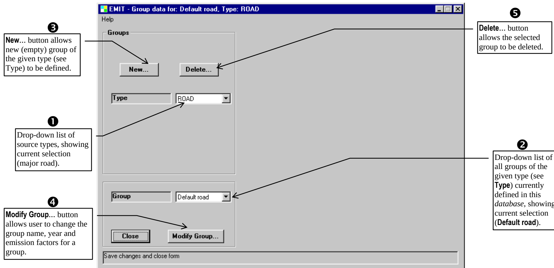
Figure 4.14 – Group data screen. This must be used to create new (empty) groups, which are subsequently populated using the EMIT Group screen.
