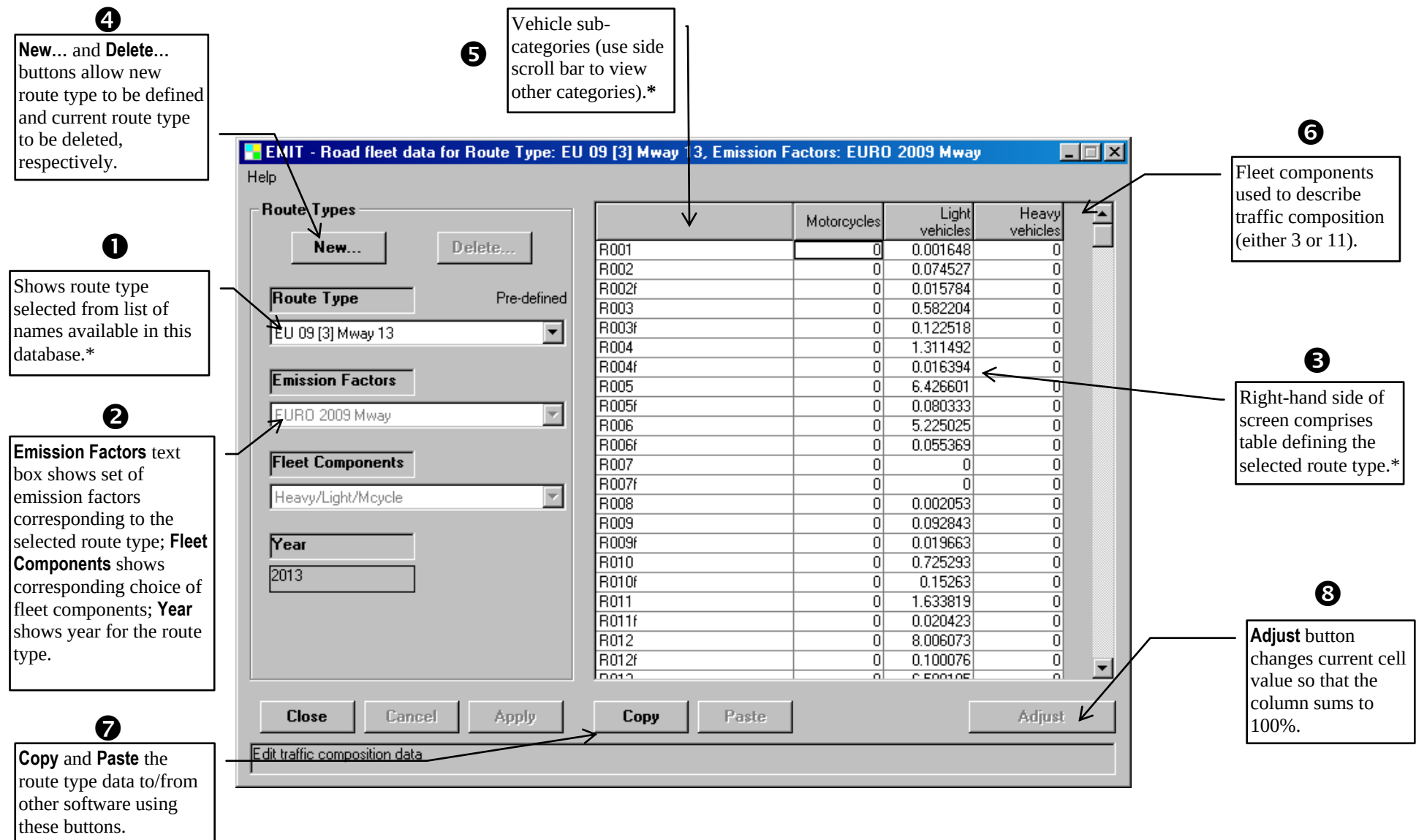
Figure 4.12 – Route type data screen (road sources). Features marked with an asterisk* are dependent on the choice of emission factors.
