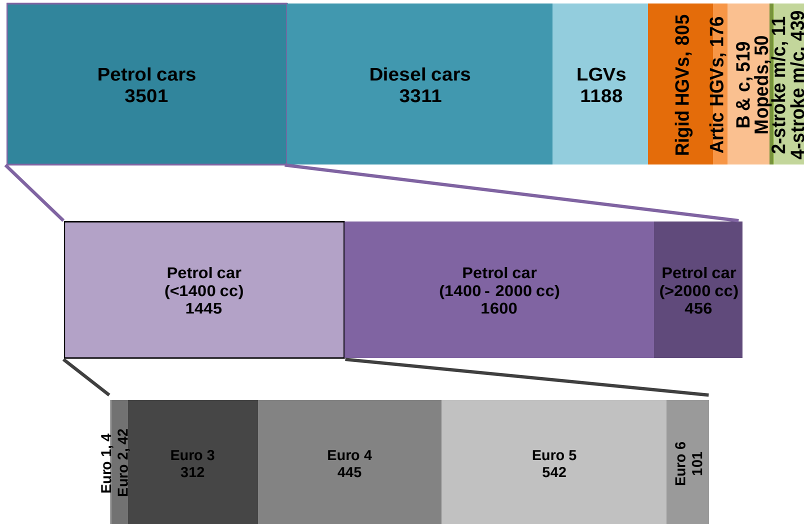
Figure A.4 – Breakdown of petrol cars in NAEI 12 Eng[3] U15 for an example AADT of 10000. For simplicity, vehicle sub-categories names are not shown.
