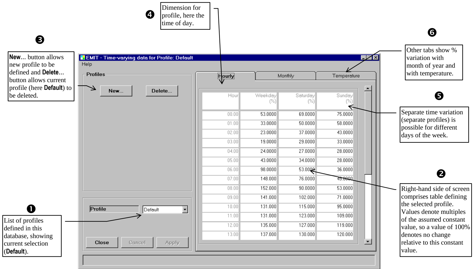
Figure 4.16 – Time-varying profiles data screen. Monthly and Temperature tabs allow variation in emission rate with month of the year and exit temperature, respectively.
