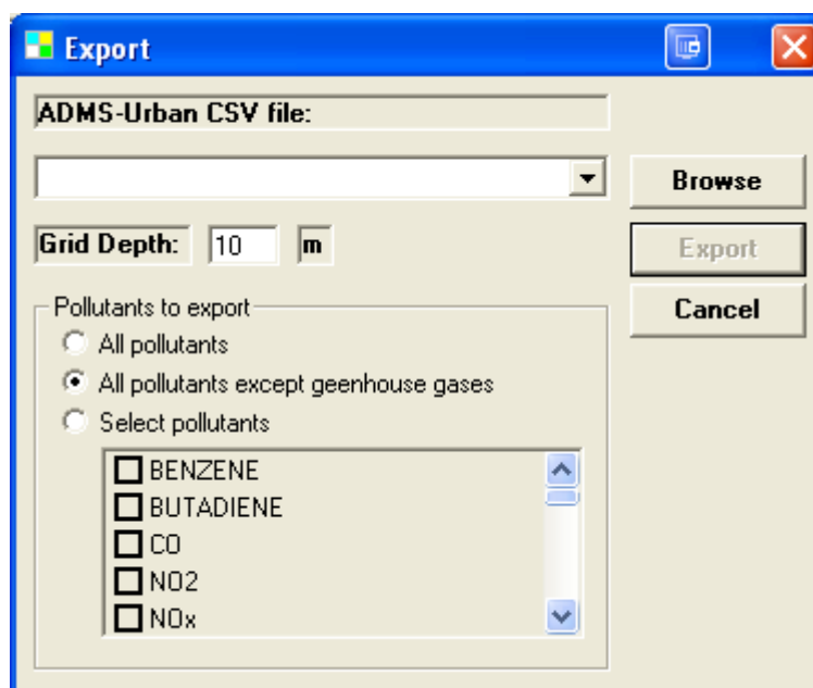
Figure 8.10 - Dialogue box for exporting grid totals to an ADMS .csv file.
